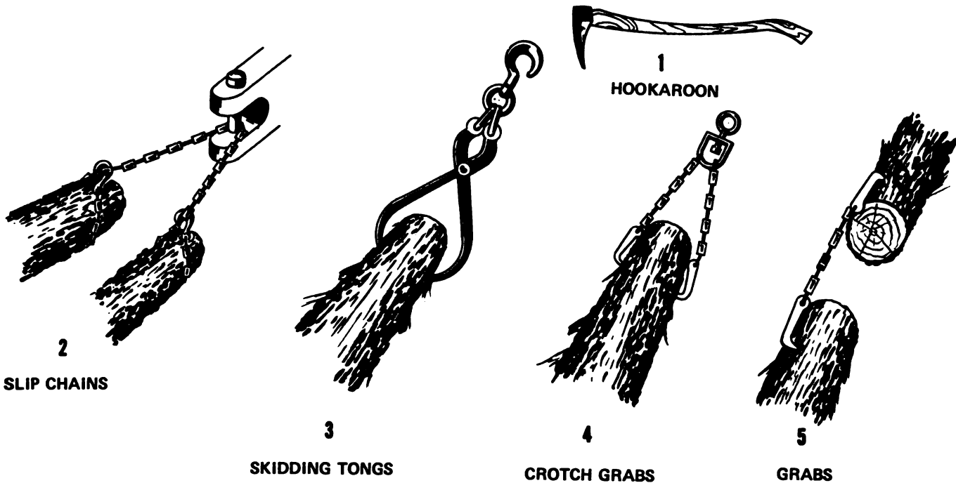
Figure 7-4. Securing logs for ground skidding.
